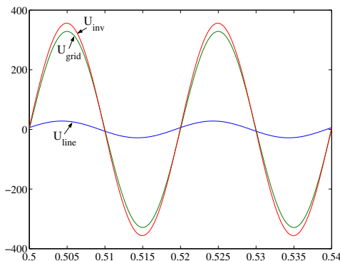
Fig. 11. Voltages @ 10 kW and \approx 0 Var
