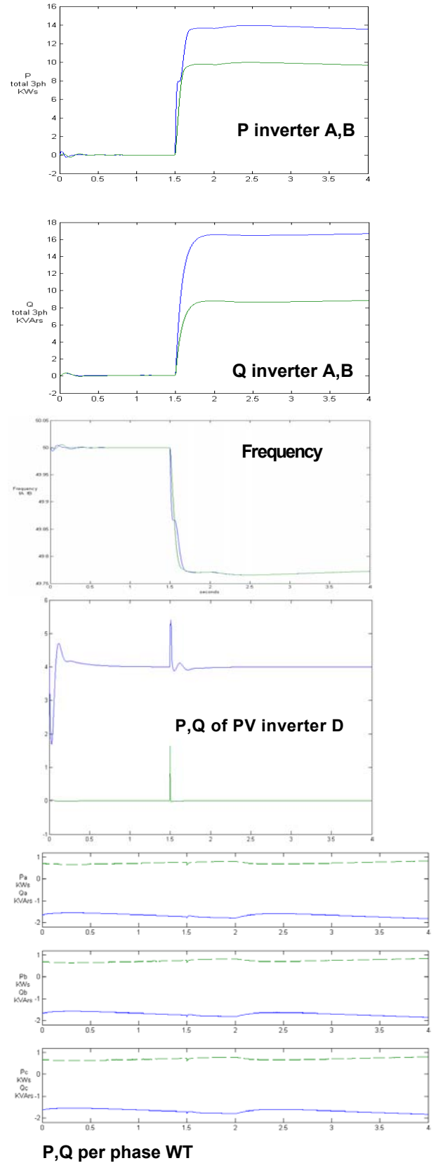
Fig. 2. Examples of results obtained by the developed simulation platform. The figures depict the response of several quantities in the microgrid following is disconnection from the main grid and under fluctuating wind generation.
