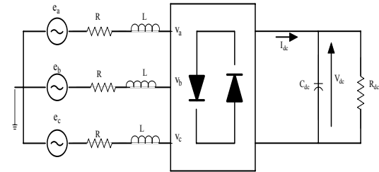
Figure 6. Circuit diagram of three-phase VSC
