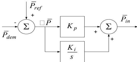
Figure 2. Load following control system model.
